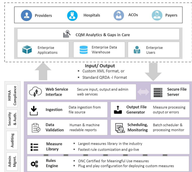
CQ-IQ: Cloud-hosted Clinical Analytics Platform
